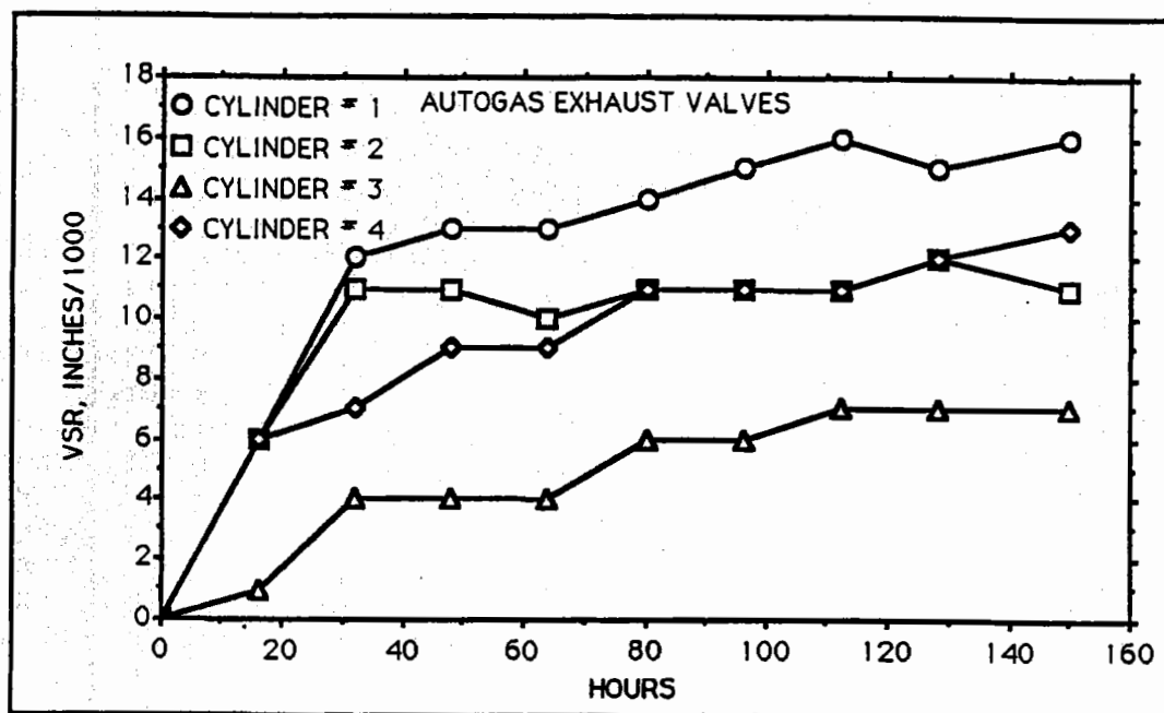
FIGURE 7. VSR in individual exhaust valves, autogas test
